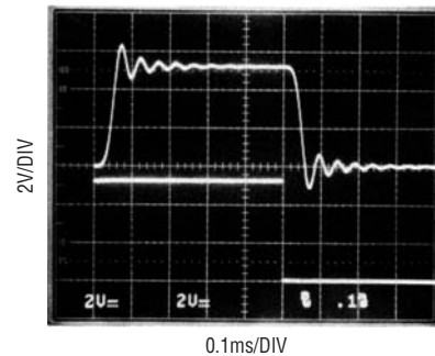
Transient Response f_{\text{CLK}} = 1\text{MHz} , Ratio = 50:1, f_C = 20\text{kHz} , V_S = \pm 7.5\text{V} , 1kHz Square Wave Input
